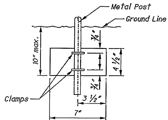
ANTI-TWIST PLATE
